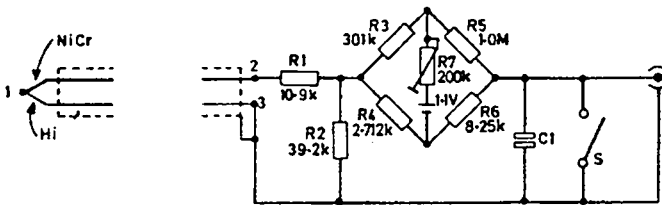
Type 54451-101L Peak-to-Peak Probe.
