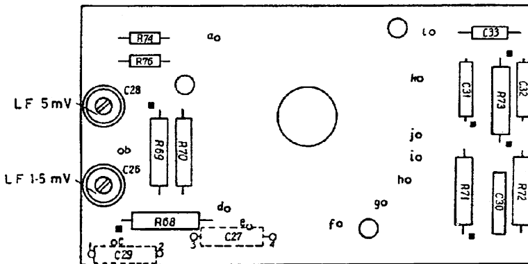
Fig 4.4 Feedback Divider (Rotary Switch) P. C. B. ( B-30-2627A )
