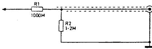
Type 54451-081C High Voltage Probe.
