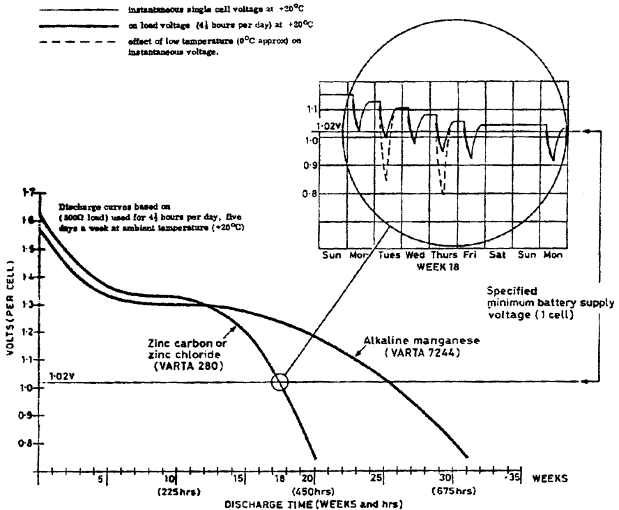
Fig 4.6 Battery discharge curves for an assumed FET Multimeter working week of 4½ hours per day, 5 days per week.
