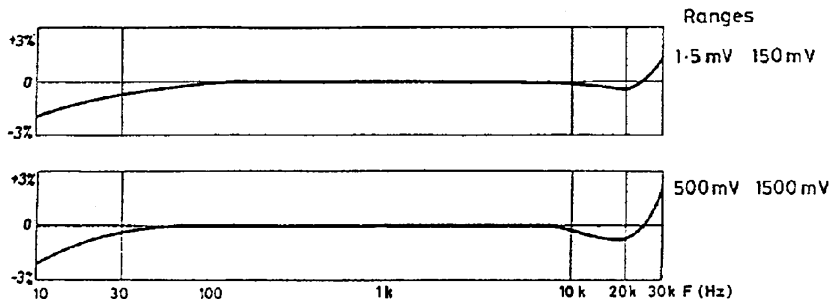
Fig. 2.2 LF Voltage Measurement Response
