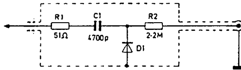
Type 54451-091E High Frequency Probe.
