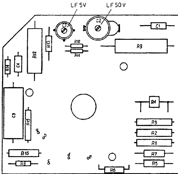
Fig 4.3 Input Divider (Rotary Switch) P. C. B. ( B-31-1549 )
