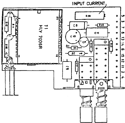
Fig. 4.1 Amplifier PCB (B-31-2005) Layout.
