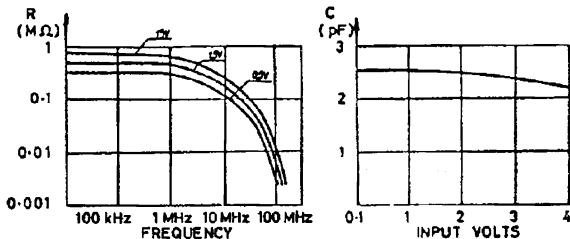
Fig. 2.4 Typical Frequency Response of RF Probe
