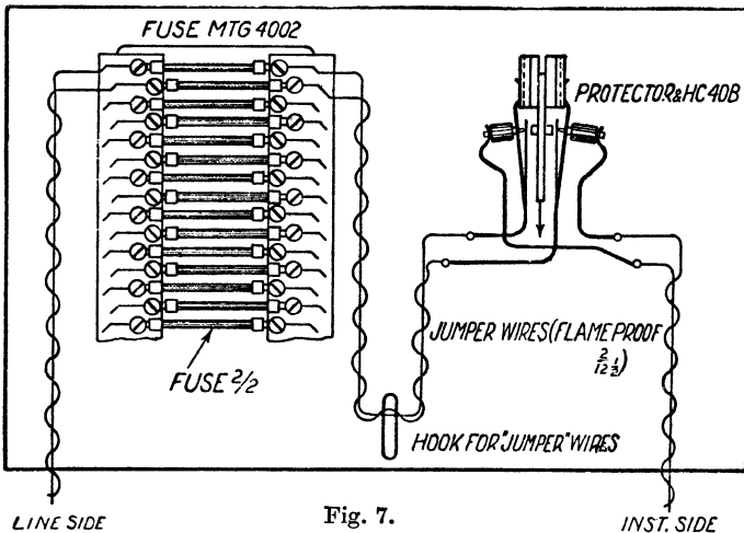
Diagram of Wiring Protectors H.C. and F\frac{4}{40} and \frac{8}{80} .
