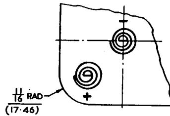
TOP VIEW SHOWING ALTERNATIVE CORNER CONSTRUCTION
