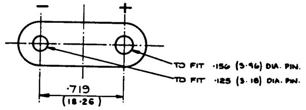
ENLARGED SOCKET DETAIL.
